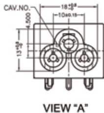
VIEW "A"
